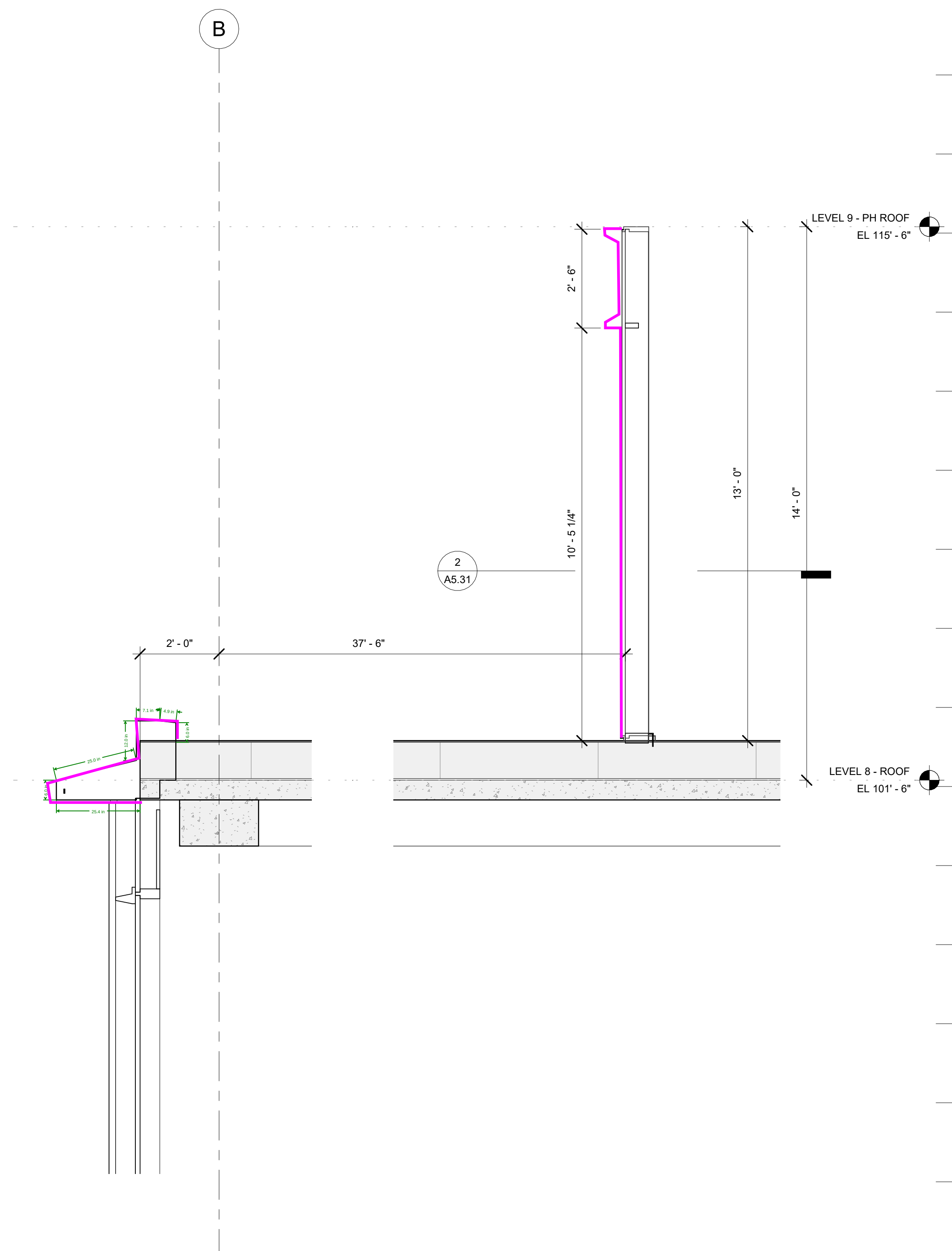
3 SECTION 1/2" = 1'-0"
